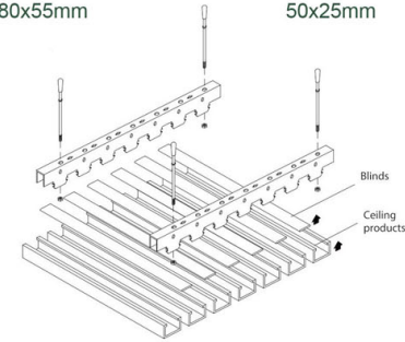
THO-8055 80x55mm
